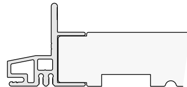
Thick Frame Cladding - PF1812
