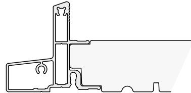
Thick Frame Cladding - PF2146
