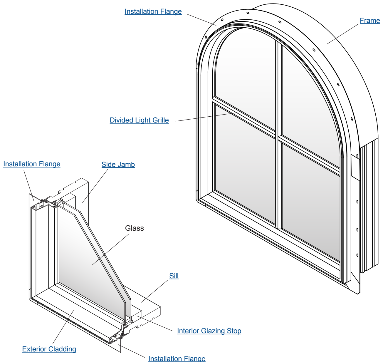
Andersen® Architectural Clad Specialty Fixed Window Unit Parts - Standard Window
