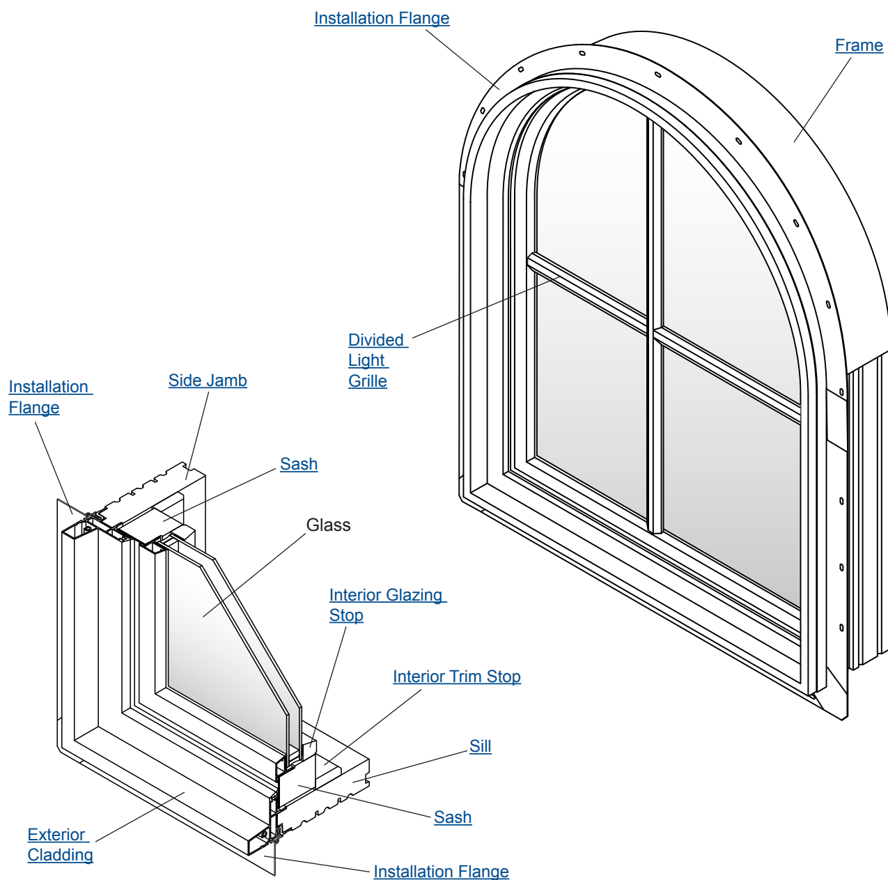
Andersen® Architectural Clad Specialty Fixed Window Unit Parts - Sash Glazed Window
