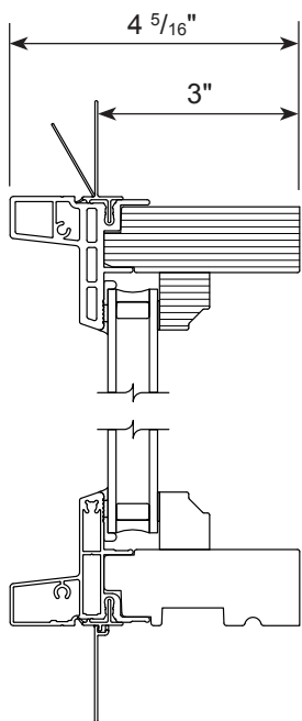
Curved Jamb
