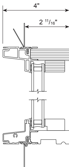
Curved Jamb
