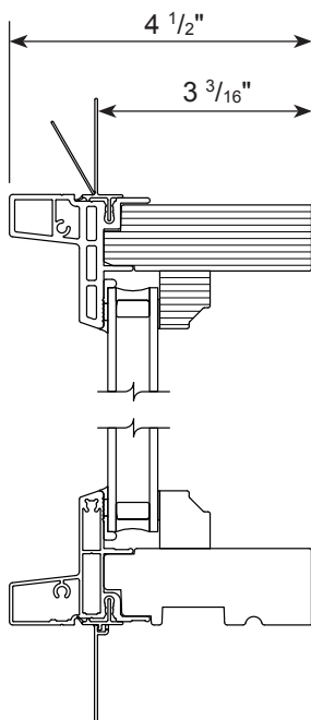
Curved Jamb
