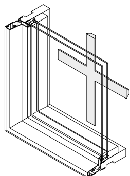
Removable Interior
