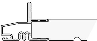
Standard Cladding - PF1073
