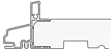
Thick Frame Cladding - PF1877
