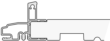
Standard Cladding - PF1875
