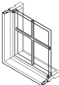
Finelight™ Between-the-Glass
