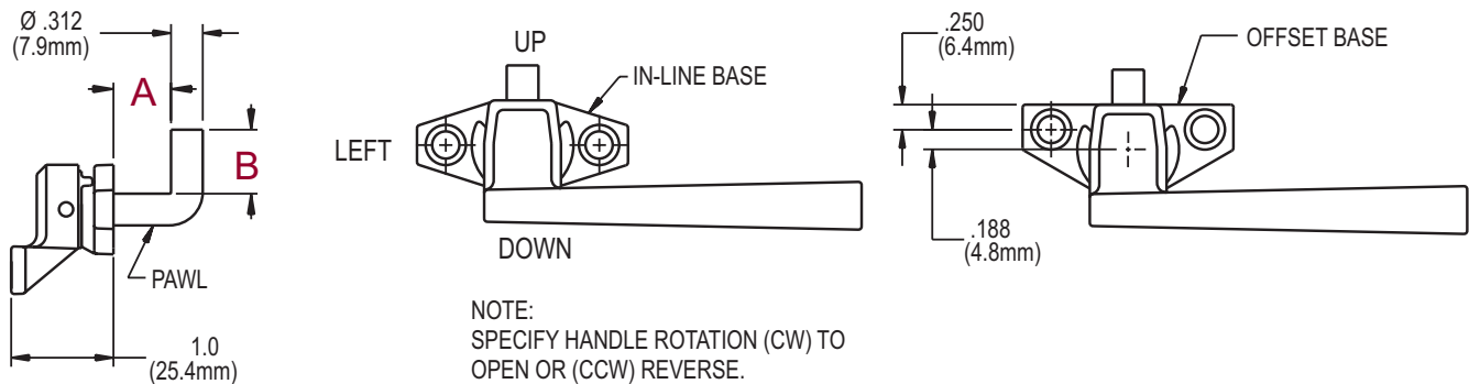
FIG. 2 TRIMLINE CAM HANDLE WITH CONCEALED PAWL
