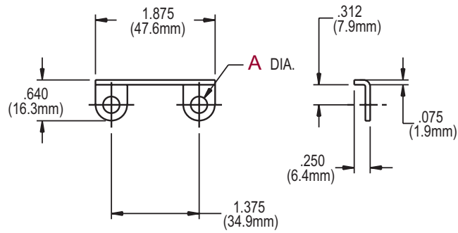
FIG. 3 20303 AND 20404 KEEPERS
