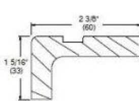
W7025-501 – Hardware Cover Lever Operator
