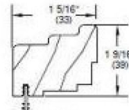
W9790 Stationary Solid Wood Jamb Stop
