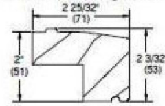
W8098 – 2" Simulated Thick Subsill
