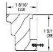
W9800 Optional Operator Solid Wood Jamb Stop
