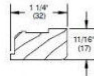
W7034 – Inside Stop Stationary and Picture Unit Head Jamb Stop Stationary and Picture Unit
