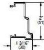
V1162 – Side Stop
