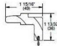
W8459 – Hardware Cover Operator
