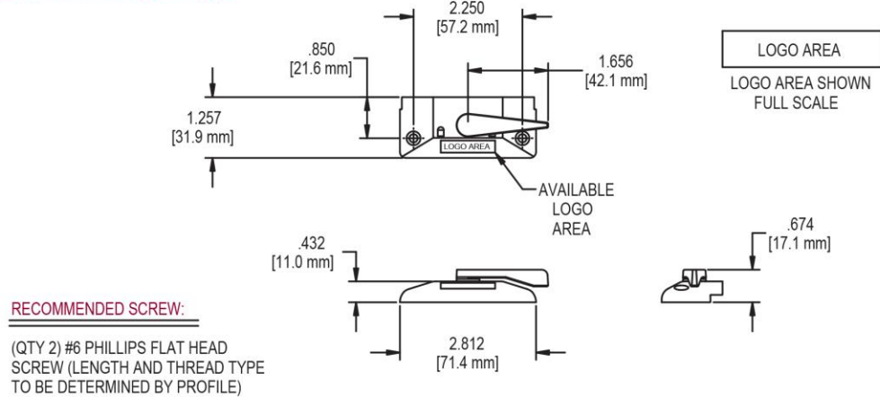
FIG. 3 C09954XX CONCEALED KEEPER
