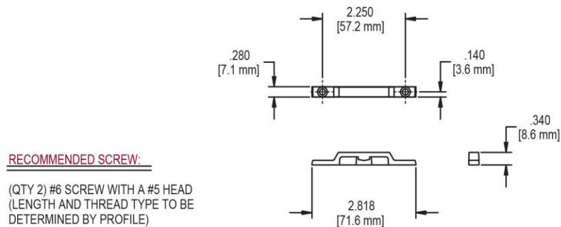
FIG. 3 C09954XX CONCEALED KEEPER
