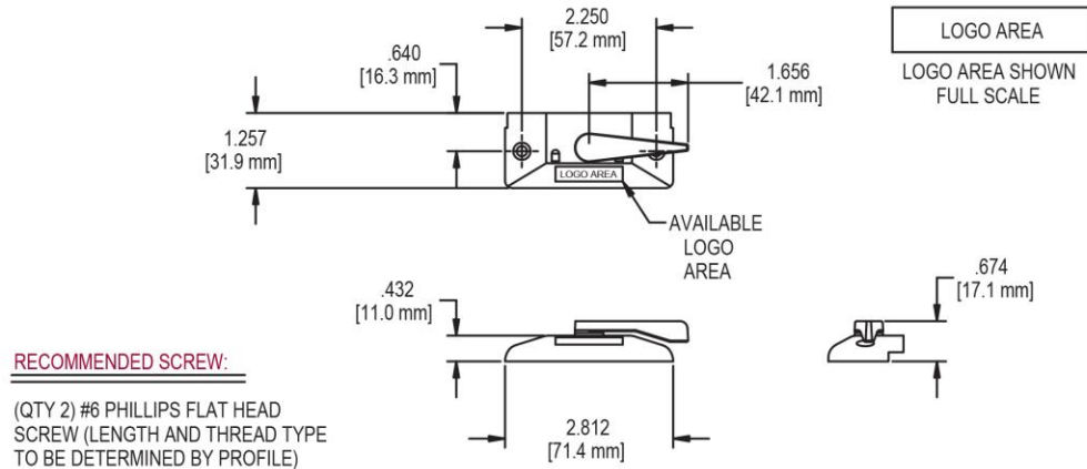
FIG. 2 A09950401XX SASH LOCK
