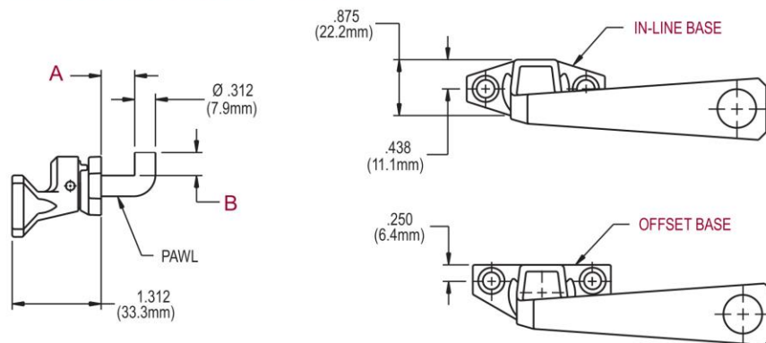
FIG. 2 CAM HANDLE WITH CONCEALED PAWL
