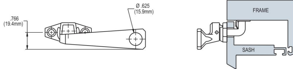
FIG. 1 APPLICATION OF CAM HANDLE WITH CONCEALED PAWL
