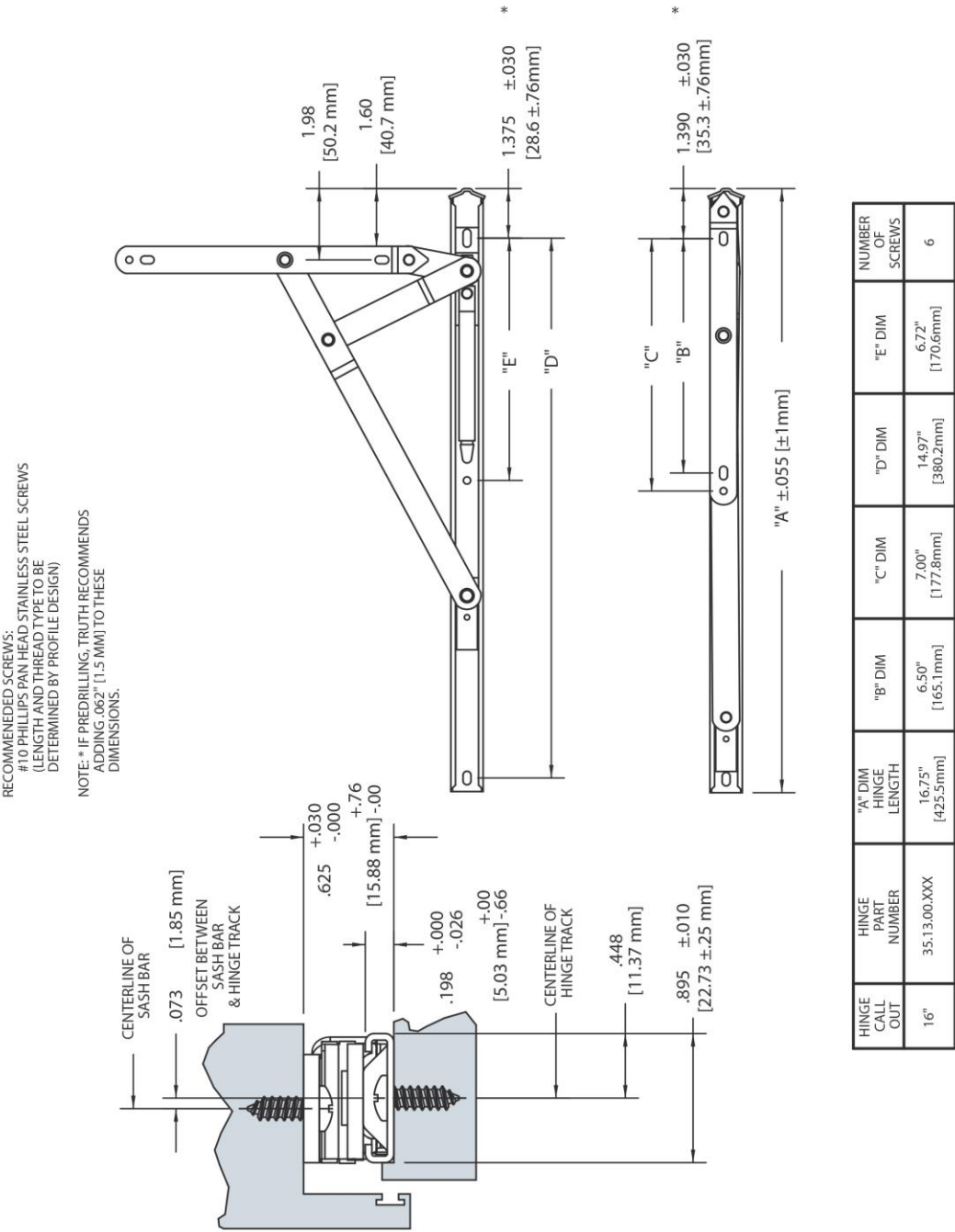
FIG. 7 TRUTH HEAVY DUTY EGRESS (90°) 4-BAR HINGE (Truth 334SS Series)
