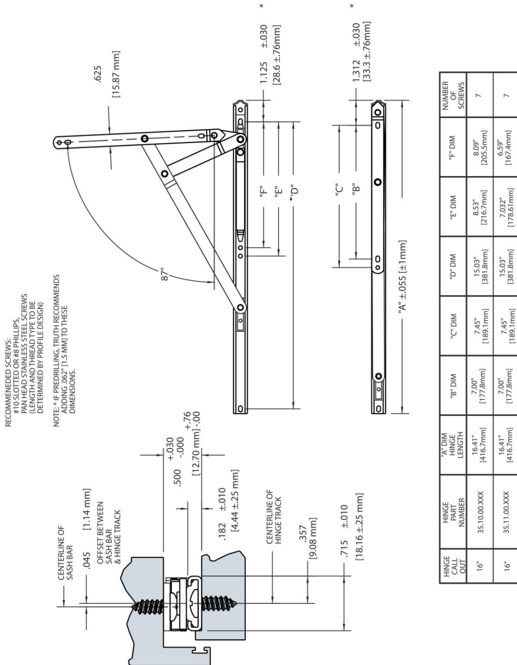
FIG. 3 TRUTH STANDARD DUTY EGRESS (90°) 4-BAR HINGE (Truth 224SS Series)
