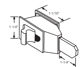
900-18069 With Indicator. For 1" Steel Door
