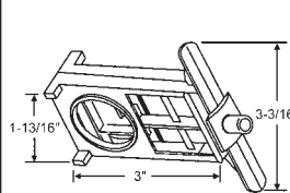
91-129 Zinc Die Cast - Unplated
