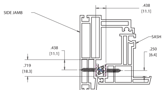
FIG. 3 22999.XX CONCEALED SNUBBER DIE CAST
