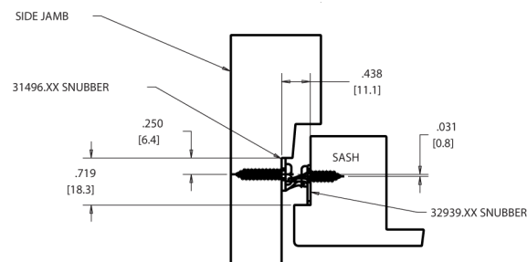
FIG. 1 32939.XX CONCEALED SNUBBER AND 31496.XX CONCEALED SNUBBER COMPRESSION
