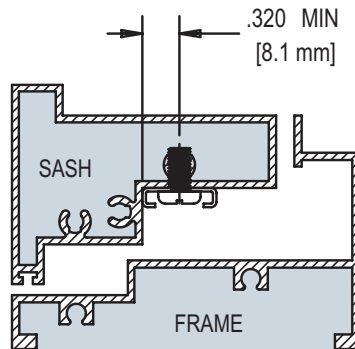
FIG. 8 APPLICATION OF MAXIM SINGLE ARM OPERATOR (CONTINUED) (SILL MOUNT VERSION) (LOW PROFILE)
