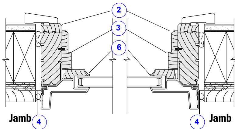
Horizontal Section Stationary Transom
