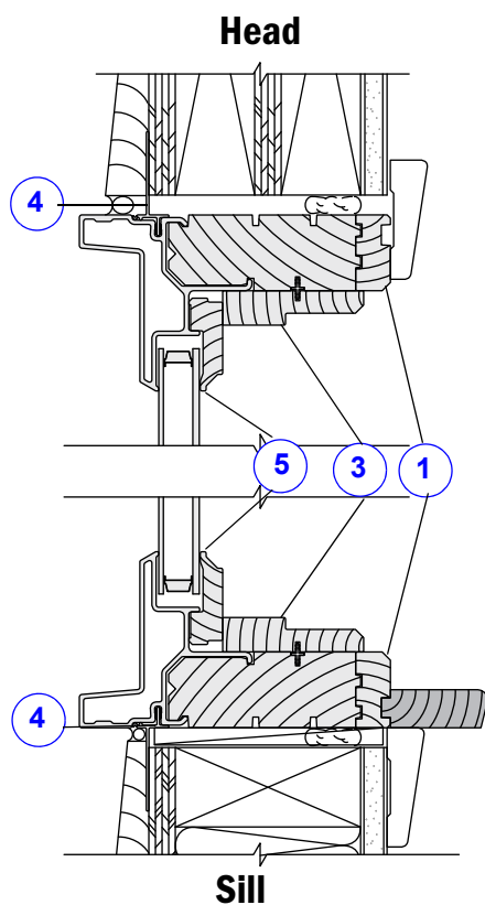
Vertical Section Stationary Transom
