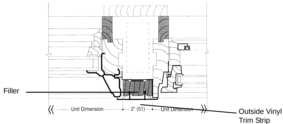
Arch Window Support Mullion
