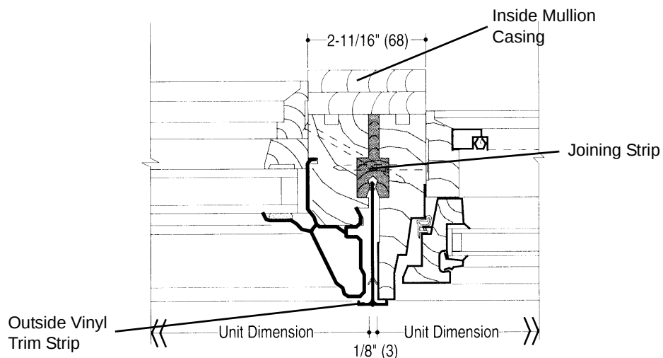
Arch Window Narrow Mullion
