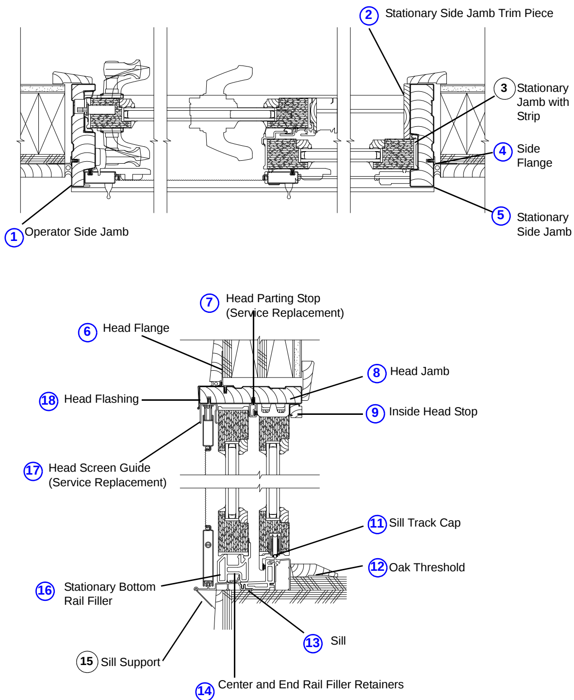
200 Narroline Doors Frame Assembly
