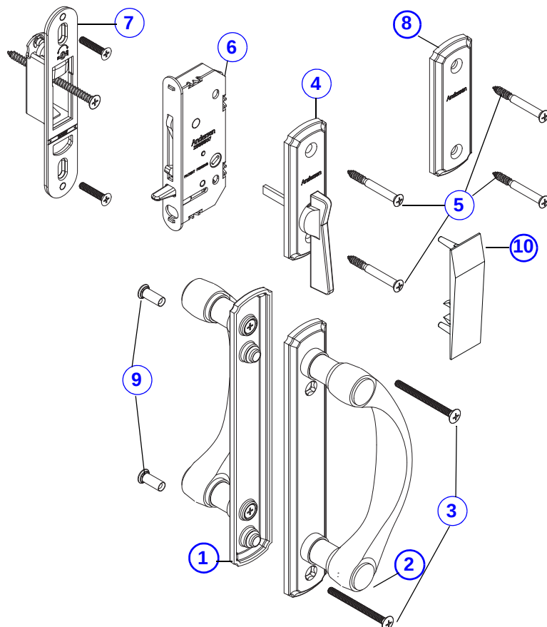
Newbury® Gliding Patio Door Hardware - Panel Trim Set
