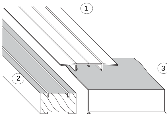
200 Series Narroline Gliding Support Mullion
