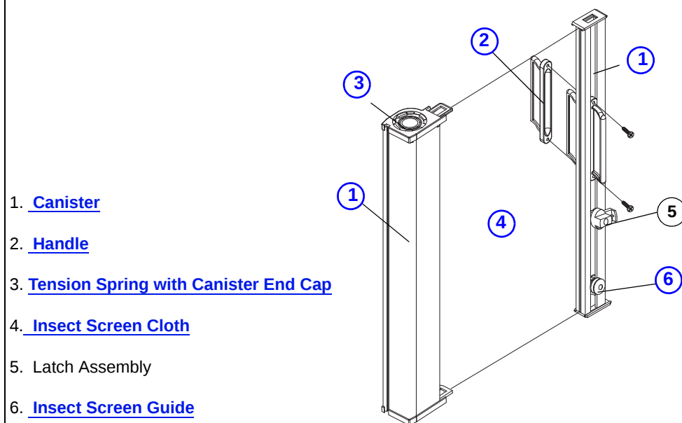
Retractable Insect Screen Unit
