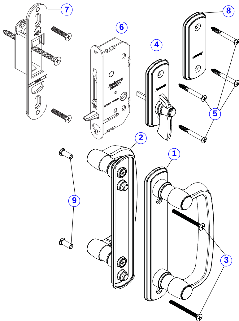
Albany Gliding Patio Door Hardware - 2-Panel Trim Set
