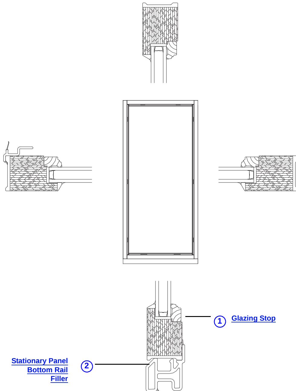
200 Series Narroline Gliding Stationary Panel (Left Hand or Right Hand)
