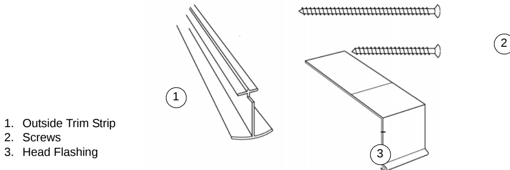
200 Series Narroline Gliding Narrow Mullion
