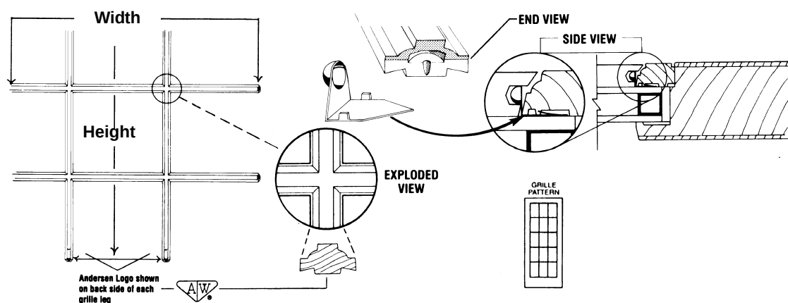
200 Series Narroline Gliding Interior Grilles - 7/8" Wood
