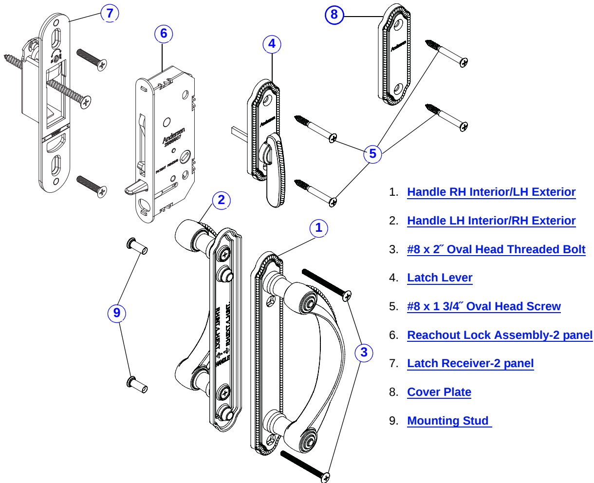
Whitmore® Gliding Patio Door Hardware - 2-Panel Trim Set
