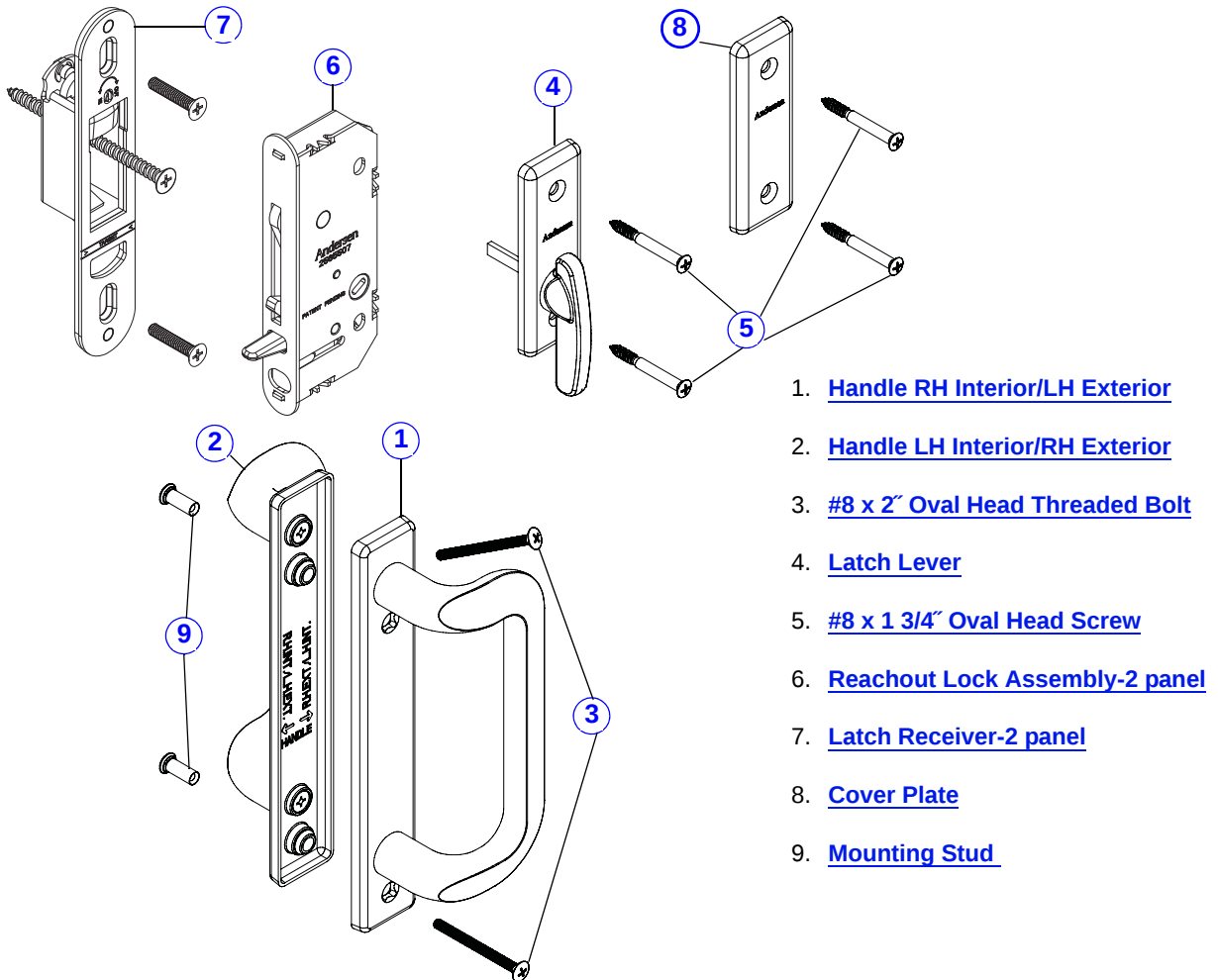
Anvers® Gliding Patio Door Hardware - 2-Panel Trim Set
