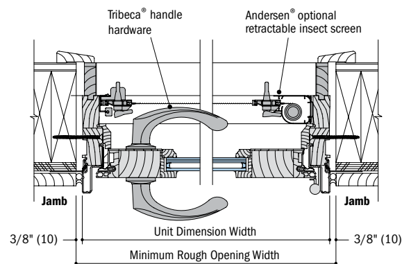
Horizontal Section High-Performance™ Low-E4® Impact-Resistant Glass
