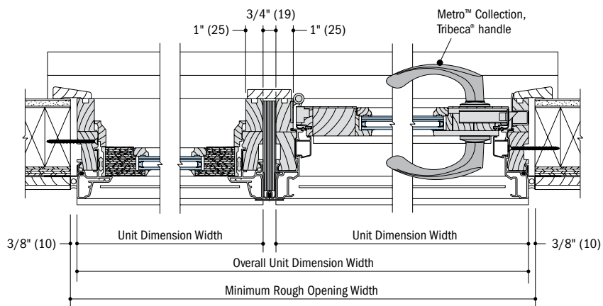
Horizontal Section Sidelight
