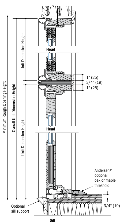
Vertical Section Transom
