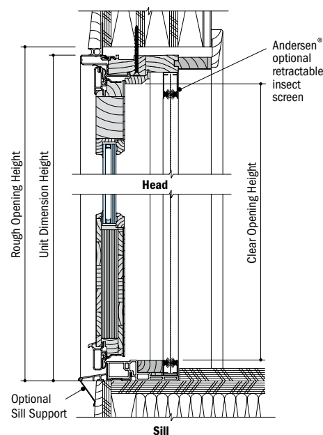
Vertical Section High-Performance™ Low-E4® Impact-Resistant Glass
