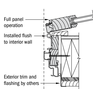
Jamb hinged patio door in 2" x 6" wall without extension jambs
