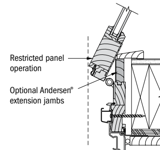
Jamb hinged patio door in 2" x 6" wall with extension jambs
