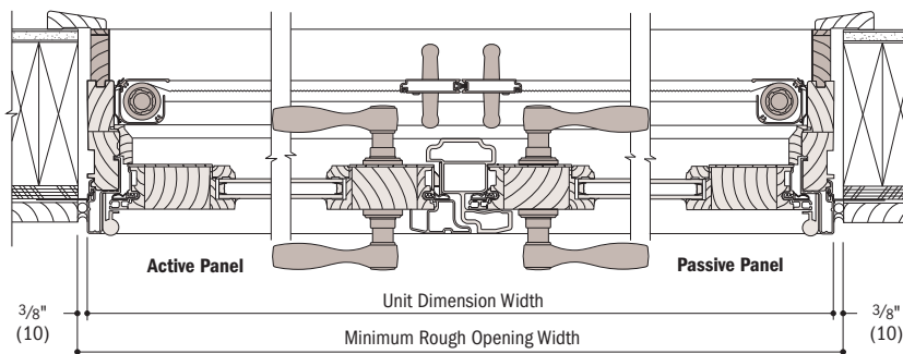
Horizontal Section 2-Panel
