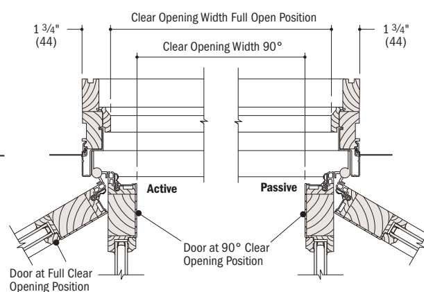
Horizontal Section 2-Panel, Active (open) and Passive (open)
