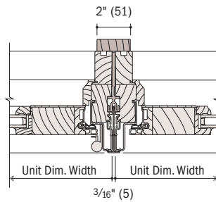
Horizontal Section Frenchwood® Hinged Outswing to Frenchwood Hinged Outswing
