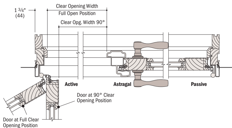
Horizontal Section 2-Panel, Active (open) and Passive (closed)
