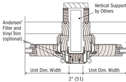
Horizontal Section Frenchwood® Hinged Outswing and Frenchwood Hinged Outswing
