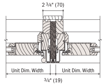
Horizontal Section Frenchwood® Hinged Outswing to Frenchwood Hinged Outswing
