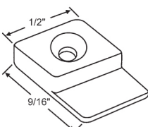
76-600 Uses 20-004 Screw
