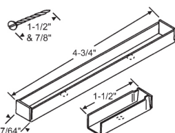
Hinge Assembly w/ Metal Bracket
