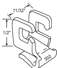
76-516 Clip On
