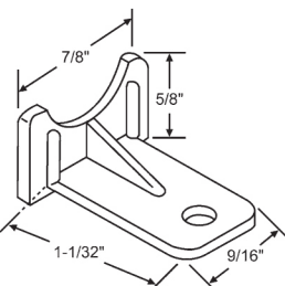
900-5013 Natural Nylon
