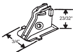
74-502 Airmaster
