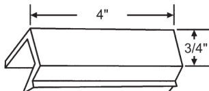
74-713 White
