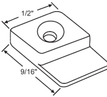
76-600 Uses Screw 20-004
