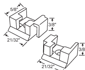
74-611 Set, LH and RH Keller
