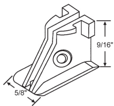
74-501
